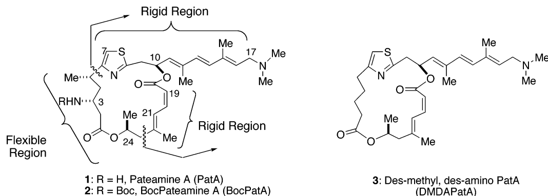
Figure 1. Structures of pateamine A (1), Boc-pateamine A (2), and des-methyl, des-amino pateamine A (DMDAPatA, 3). Also shown are the putative binding (rigid regions) and scaffolding (flexible) domains.
